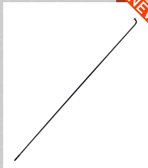
TR-SPK-112 Material: Steel C45 Type: J-Bend Gauge: 13G-2.3mm Length: 140mm to 300mm Colour: Galvanized Black
