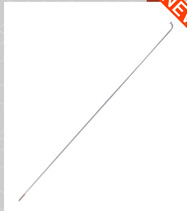
TR-SPK-222 Material: Stainless Steel Type: J-Bend Gauge: 13G-2.3mm Length: 140mm to 300mm Colour: Silver
