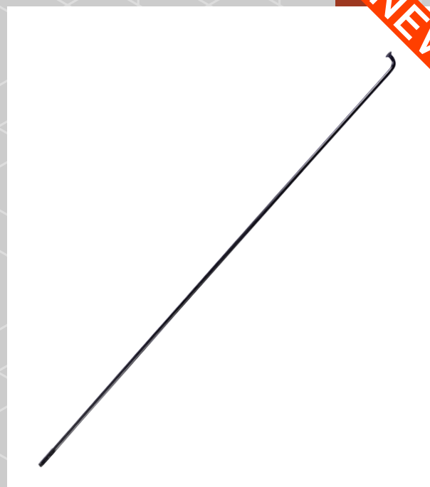
TR-SPK-111 Material: Steel C45 Type: J-Bend Gauge: 14G-2mm Length: 140mm to 300mm Colour: Galvanized Black
