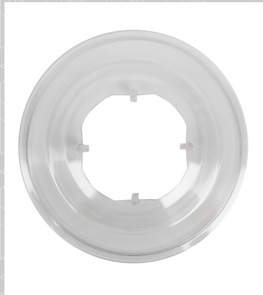
TR-SPP-111 Product: Spoke Protector Type: Cassette Hub Type 4 Teeth 28H-32H Compatible Material: PC Outer Diameter Ø: 155mm Teeth to Teeth: 39mm Colour: Transparent
